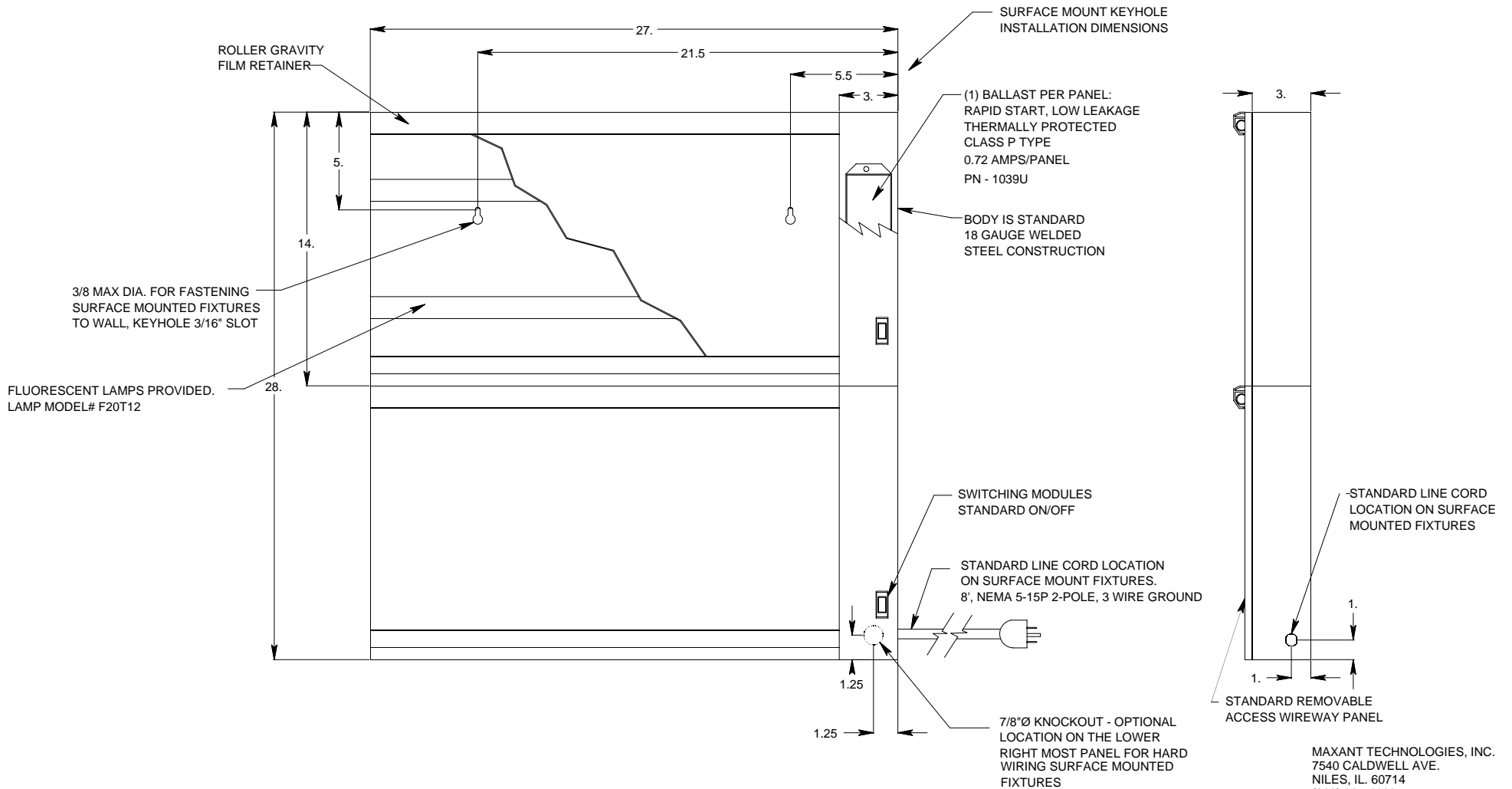
FRONT VIEW
