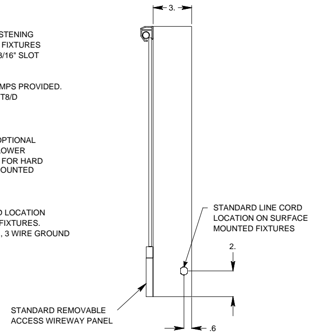
RIGHT VIEW
